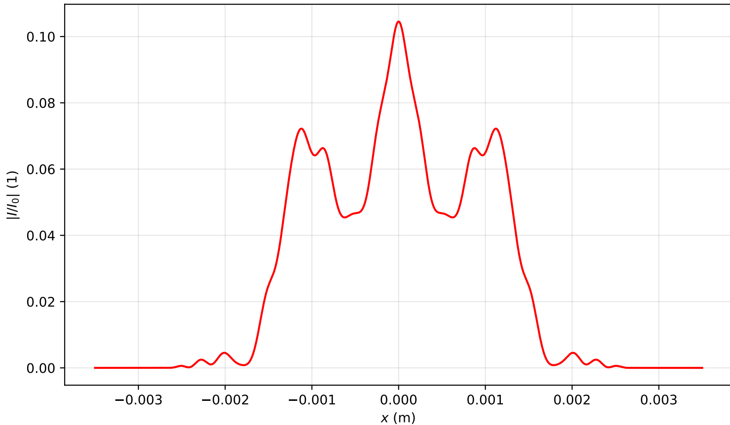
Intensity profile I(x, y = 0, z = 2.866)/I_0 , P_{in}=6.0P_{cr} , artificial time
